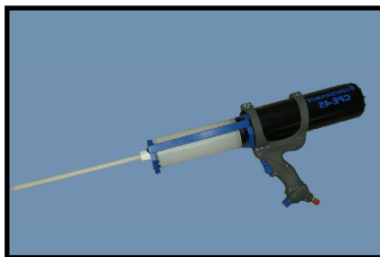
CPE-45 4" Pneumatic Cylinder Ergonomic Handle 600ml x 600ml factory set-up, 750ml x750ml, 300ml x 300ml, conversion parts includedd.
